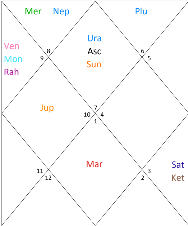
Lagna Chart
