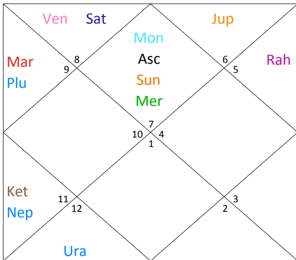
Moon Chart
